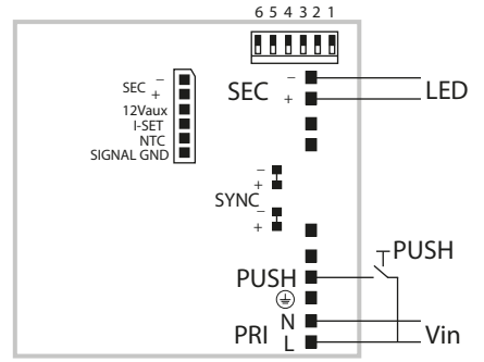
PUSH diagram - Collegamento PUSH
